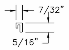
② GLAZING COMPOUND STOP EXTRUDED VINYL 0.085" THICK
