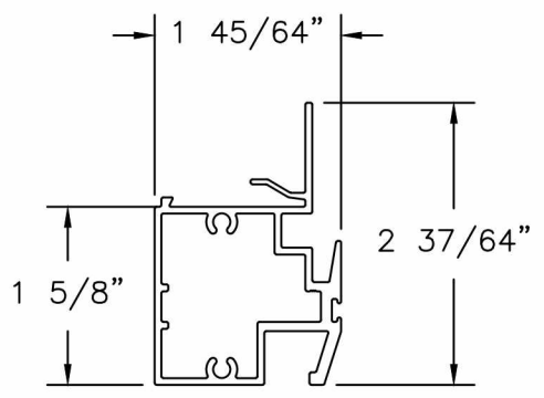
④ IMPACT MEETING RAIL EXTRUDED ALUMINUM 6063-T6 0.063" THICK
