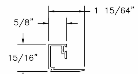
⑤ 5/16" IMPACT GLAZING BEAD EXTRUDED ALUMINUM 6063-T6 0.062" THICK
