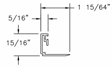
① 5/8" INS IMPACT GLAZING BEAD EXTRUDED ALUMINUM 6063-T6 0.062" THICK
