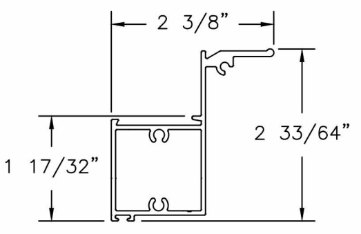
① VENT S.H. VENT SILL EXTRUDED ALUMINUM 6063-T6 0.063" THICK
