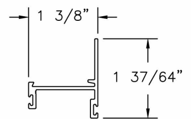
③ IMPACT VENT JAMB EXTRUDED ALUMINUM 6063-T6 0.062" THICK
